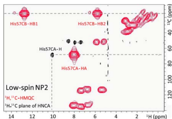
Figure 5. ^1\text{H} - ^{13}\text{C} -HMQC (red) and HNCA plane (black) of low-spin NP2 in 50 mM sodium acetate, pH 5.0, at 305 K. The ^1\text{H} - ^{13}\text{C} -HMQC spectrum was acquired with a total recycle time and a delay for transfer of 250 and 1 ms, respectively, and the ^1\text{H} - ^{13}\text{C} -plane of the HNCA spectrum was acquired with a total recycle time of 700 ms. The two small HMQC cross peaks at larger ^1\text{H} chemical shift than the two His57CB-HB cross peaks are those arising from the A heme orientation. Cross peaks corresponding to His57 are labeled in the figure whereas the remaining cross peaks correspond to ^1\text{H} - ^{13}\text{C} correlations of histidine residues other than His57.
