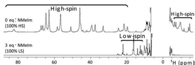
Figure 2. 600 MHz {}^1\text{H} NMR spectra of high-spin (top) and NMeIm-bound low-spin (bottom) NP2 in 50 mM sodium acetate, pH 5.0, at 305 K. FIDs were processed with a preexponential factor of 15 Hz. The assignments of all of the paramagnetically shifted {}^1\text{H} resonances of the high-spin complex are well-known, 18 and are provided in Supporting Information Figure S3 (top). Those of the low-spin NMeIm complex are also well-known. 70
