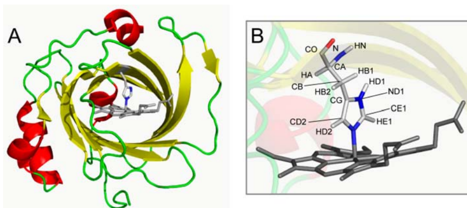
Figure 1. (A) Cartoon representation of the structure of \text{NH}_3 -bound NP2 (PDB ID 2EU7) showing the heme group and His7 rendered as sticks. (B) Zoom on iron-bound His7, indicating the atom names used throughout this work. NP2 contains three additional histidines, His26, His119, and His138, all of which are on the outside surface of the \beta -barrel and do not interact with the heme. The figure was rendered with PyMol version 0.96 (DeLano Scientific).
