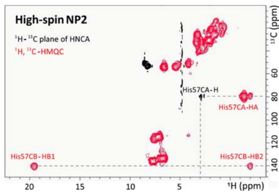
Figure 4. ^1\text{H}-^{13}\text{C} -HMQC (red) and HNCA ^1\text{H}-^{13}\text{C} -plane (black) of high-spin NP2 in 50 mM sodium acetate, pH 5.0, at 305 K. The ^1\text{H}-^{13}\text{C} -HMQC spectrum was acquired with a total recycle time and a delay for transfer of 250 and 1 ms, respectively, and the ^1\text{H}-^{13}\text{C} -plane of the HNCA spectrum was acquired with a total recycle time of 700 ms. Cross peaks corresponding to His57 are labeled in the figure whereas the remaining cross peaks correspond to ^1\text{H}-^{13}\text{C} correlations of histidine residues other than His57 (i.e., His26, His119, and His138, not affected by the paramagnetism of the heme iron).
