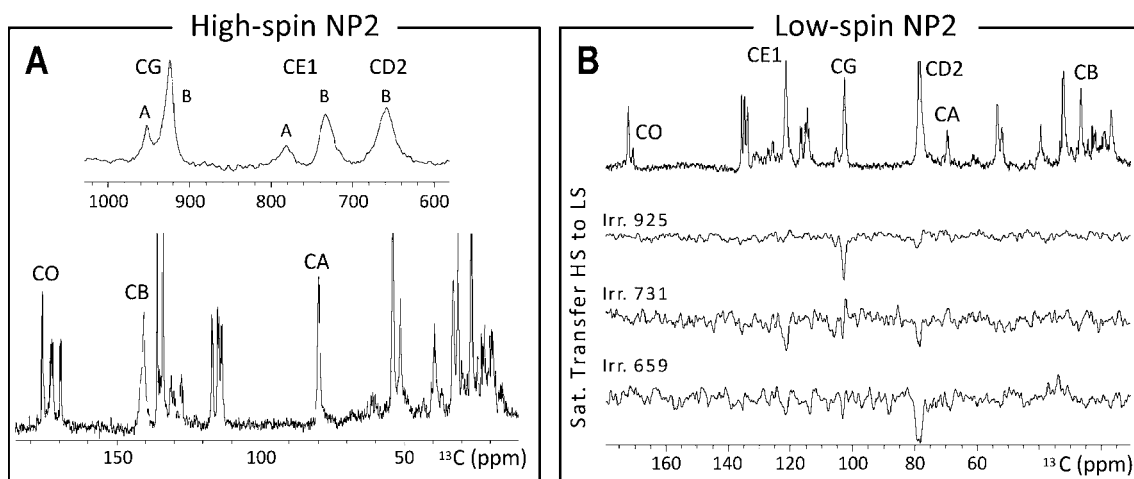
Figure 3. 150 MHz ^{13}\text{C} NMR spectra of high-spin (A) and low-spin (B) ^{13}\text{C},^{15}\text{N} -His-labeled NP2 in 50 mM sodium acetate, pH 5.0, at 305 K. For spectra corresponding to the lower shielding and diamagnetic regions of the high-spin NP2, 400k and 20k transients were accumulated and were processed with preexponential factors of 400 and 20 Hz, respectively, whereas for the low-spin NP2 spectrum 20k transients were accumulated and processed with a preexponential factor of 20 Hz. Saturation transfer difference experiments were carried out on a sample containing both the high- and low-spin forms of the protein in a ca. 1:1 ratio and using a delay for transfer of 40 ms. For difference spectra shown here 120k transients were accumulated and processed with a preexponential factor of 100 Hz. Labels for His57 carbons (CE1, CD1, CG, CB, CA, etc.) are provided in Figure 1B. Labels (A, B) in panel A (top) correspond to the two different heme orientations.
